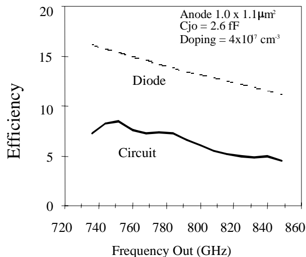
Figure 6. Calculated efficiency of new 800 GHz doubler.
