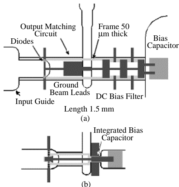
Figure 1. 400 GHz doublers. (a) Original. (b) Next generation.
