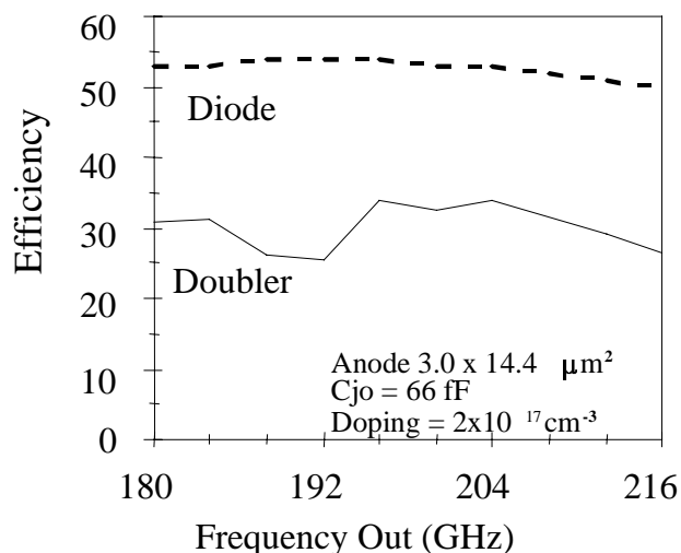
Figure 4. Calculated efficiency of new 200 GHz doubler.
