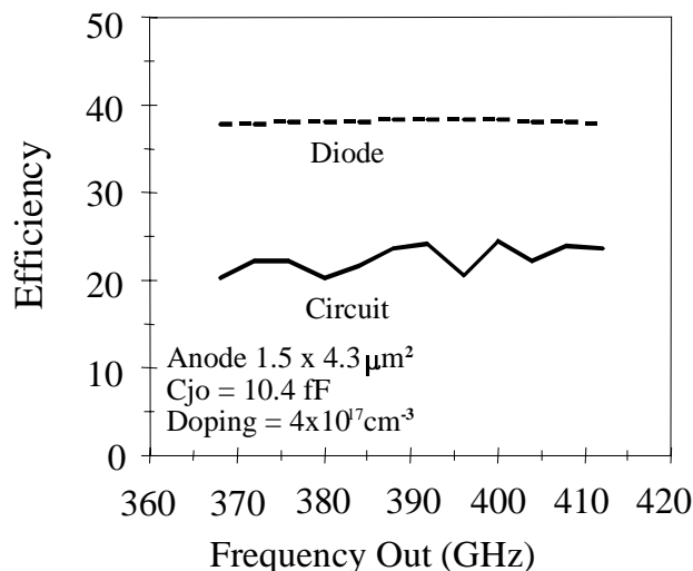
Figure 5. Calculated efficiency of new 400 GHz doubler.
