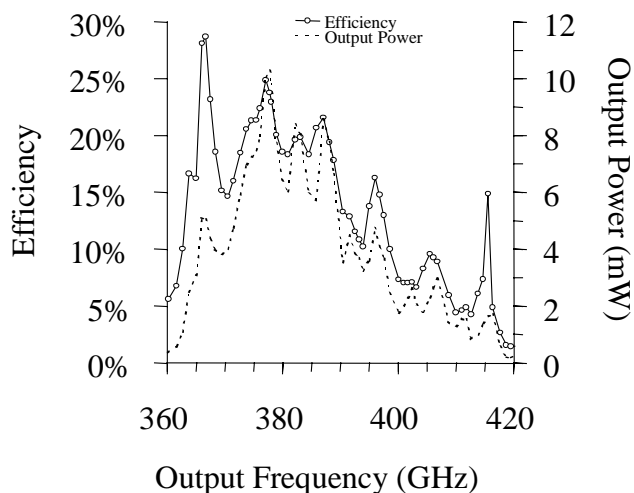
Figure 3. Measured efficiency, output and input power of 400 GHz doubler.
